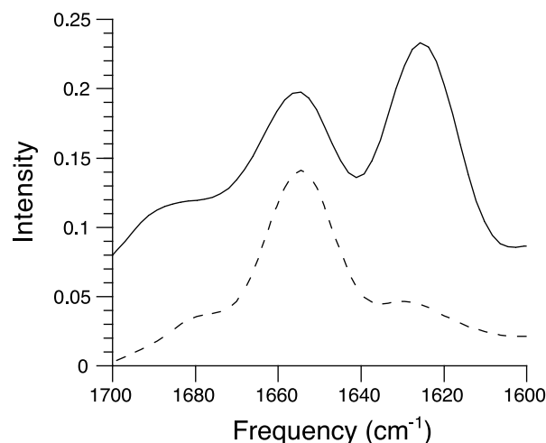
FIGURE 2 Transmission FTIR spectra of the glyophorin A transmembrane peptide. The spectrum obtained after detergent dialysis exhibits two components at 1655 and 1625\text{ cm}^{-1} (solid curve), which correspond to \alpha -helical and extended \beta -structure, respectively. Only the helical band at 1655\text{ cm}^{-1} (dashed curve) is observed after sucrose gradient purification.
