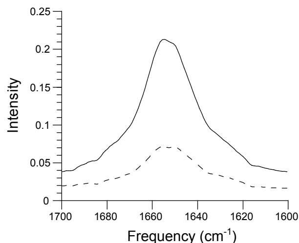
FIGURE 4 Polarized FTIR spectra of the glycoporphin A transmembrane peptide using parallel (solid line) and perpendicular (dashed line) polarized light. The peptide was reconstituted by detergent dialysis and purified on a 10–40% sucrose gradient. The reconstituted membranes were layered on the ATR crystal from a \text{D}_2\text{O} solution. The dichroic ratio of the 1655\text{ cm}^{-1} band is 3.4.
