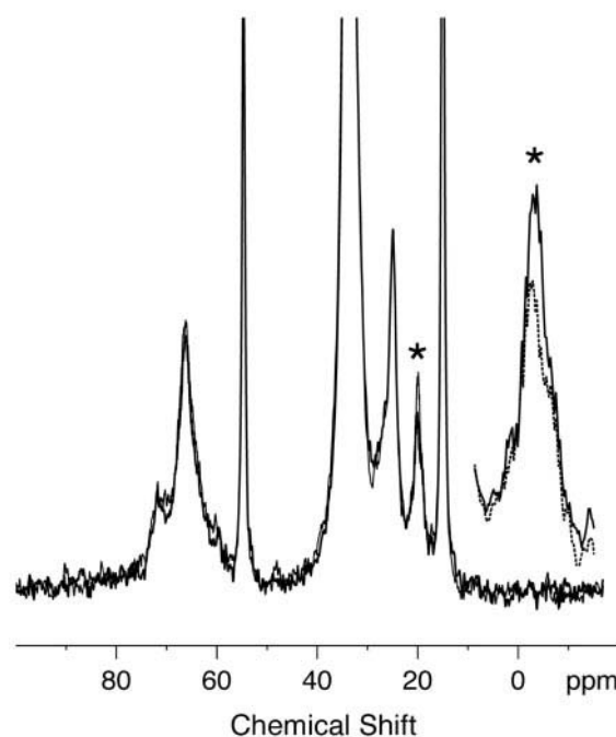
FIGURE 6 ^{13}\text{C} REDOR spectra of \text{U-}^{13}\text{C} Thr-87-labeled glycoporphin A complexed with ^{15}\text{N} -Ile-88-labeled glycoporphin A. The full and reduced spectra are overlaid. The inset shows the \gamma\text{-CH}_3 resonance at 19.6 ppm. The reduced spectrum was obtained with 48 rotor cycles of ^{15}\text{N} dephasing pulses. The MAS frequency was maintained at 4000 \text{ Hz} \pm 5 \text{ Hz} . The proton decoupling field strength was 83 kHz.
